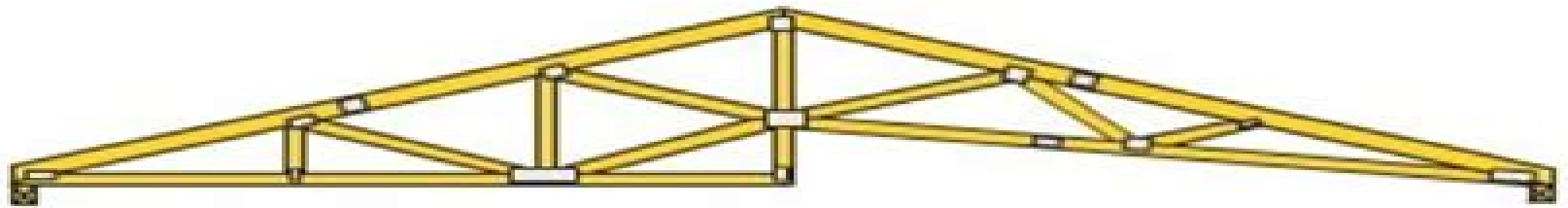
Vault - Two Bearing Points
