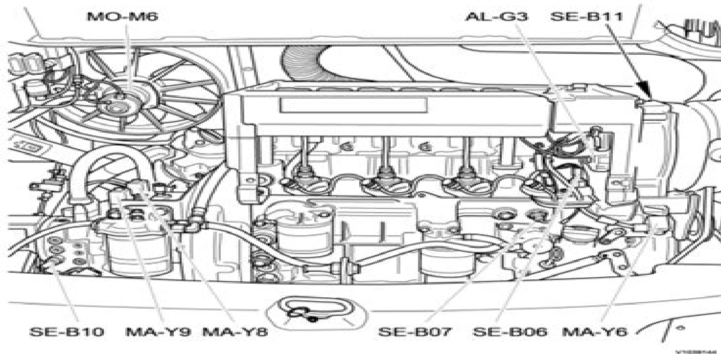
Figure 302 Electrical components, engine side
