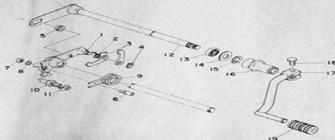
Fig. 1.10 Gearchange mechanism
