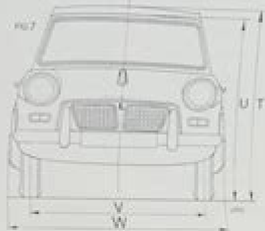
Fig. 7. Model 1200 End Elevation
