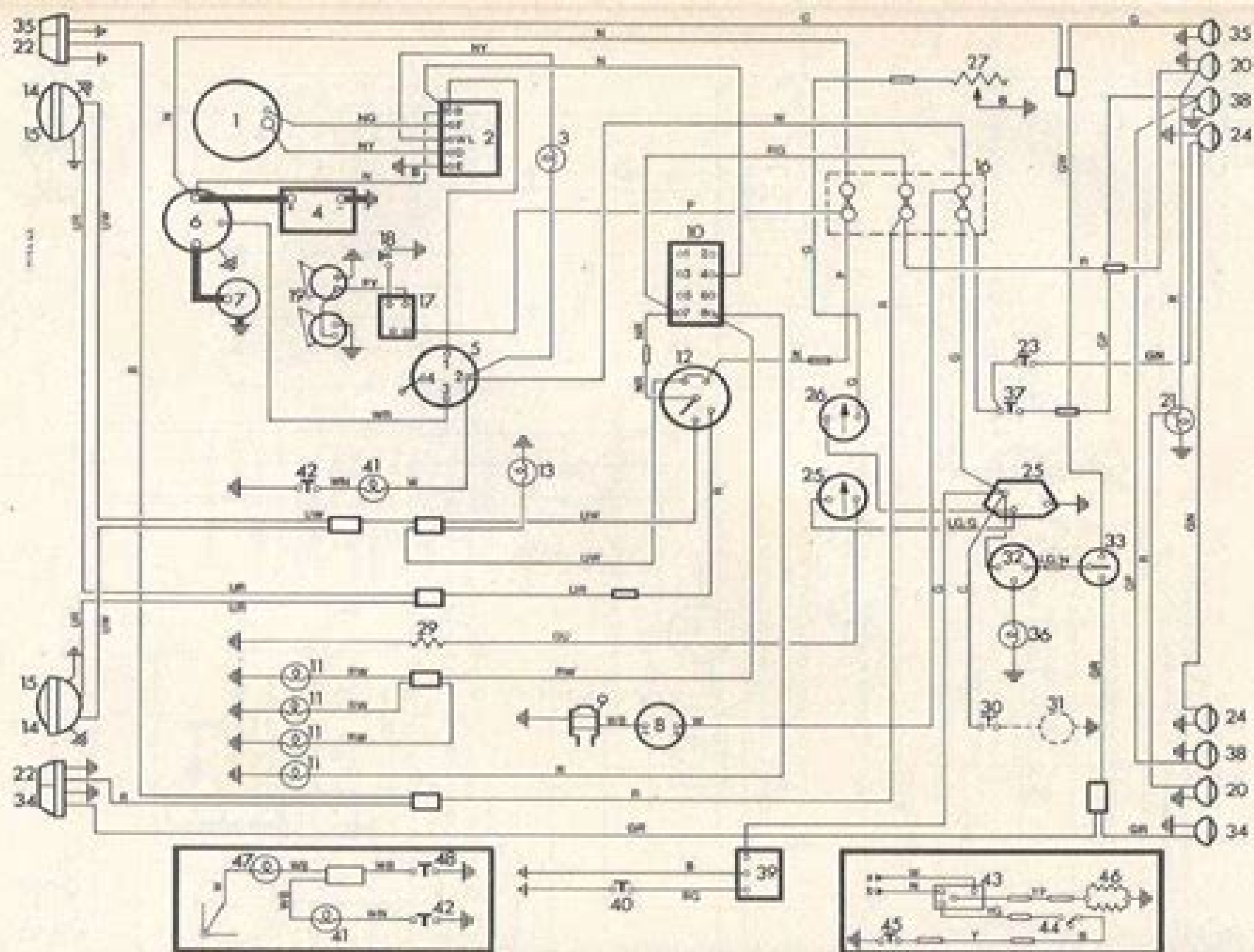
Fig. 10.54 Wiring diagram for Spitfire Mk III negative earth RHD and LHD
