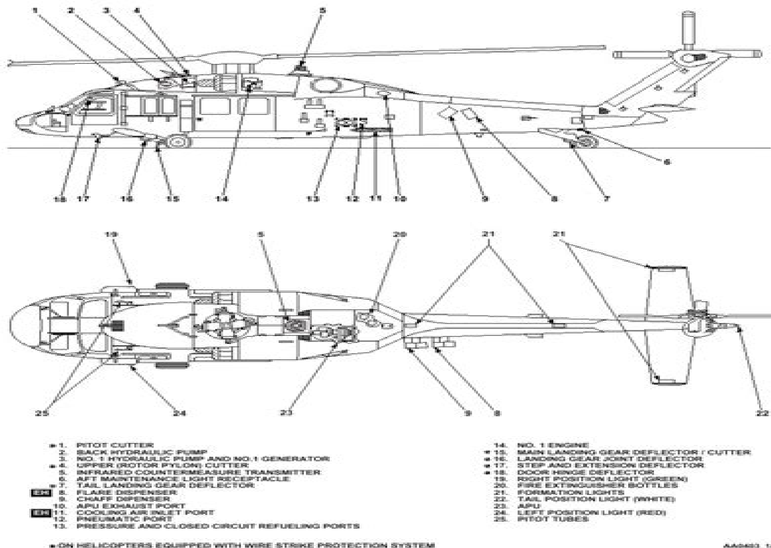
Figure 2-1. General Arrangement (Sheet 1 of 2)
