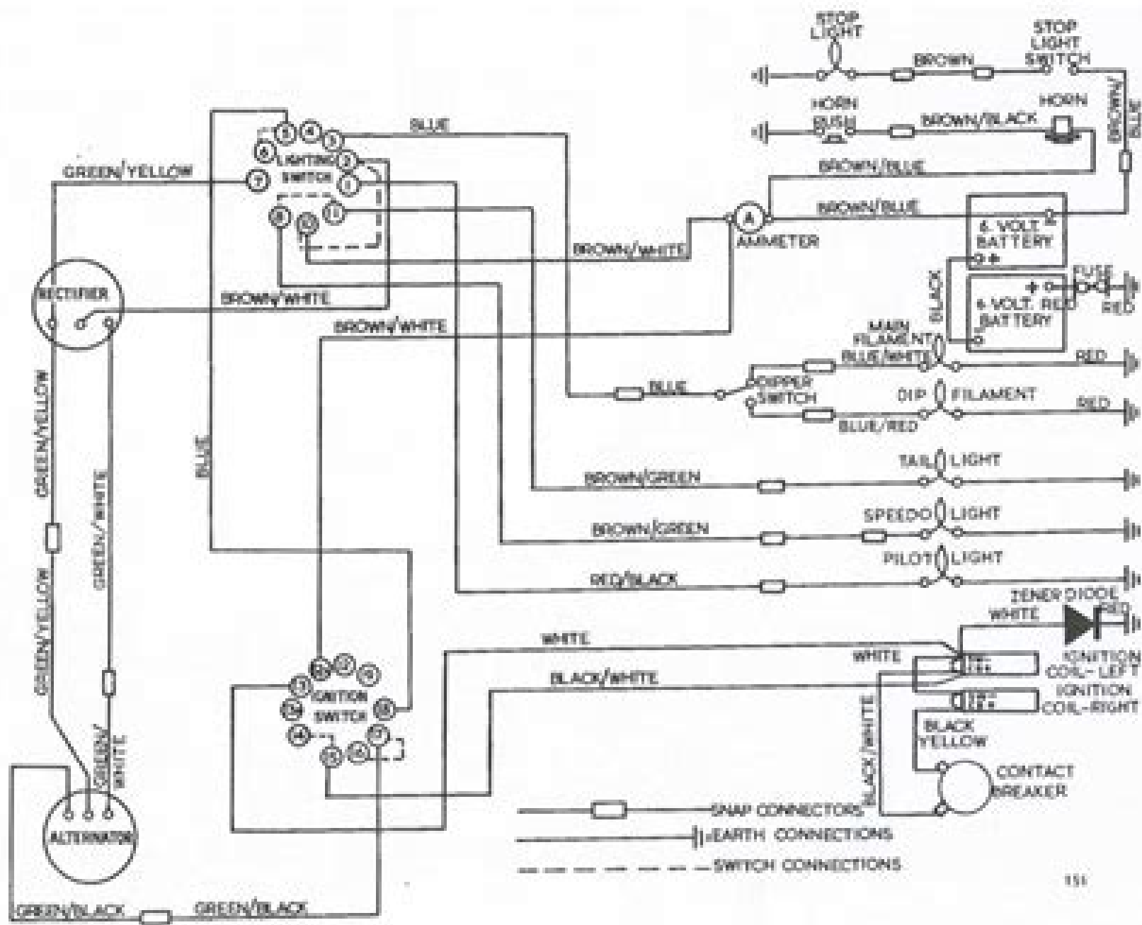
Fig. H37. Wiring diagram—Coil Ignition 12V models with Zener Diode and 3 rate charge control Before engine number DUJ.34875
