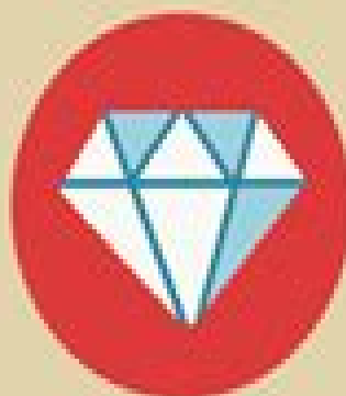
Inorganic Chemistry
