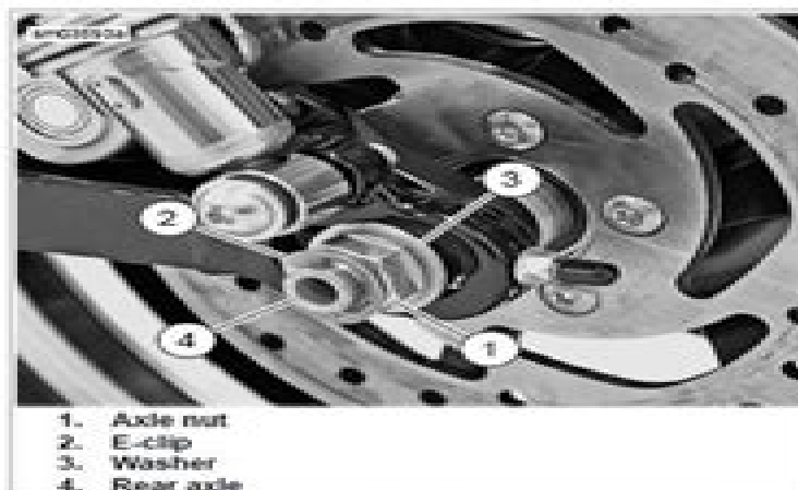
Figure 2-11. Rear Wheel Mounting
