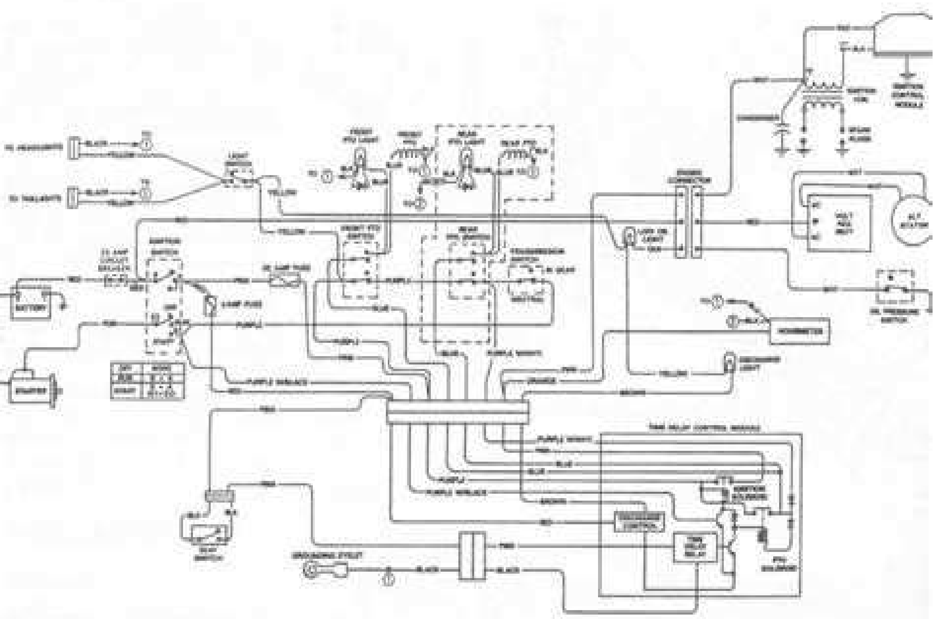
D6-23-Wiring diagram for Models 318 and 420.
