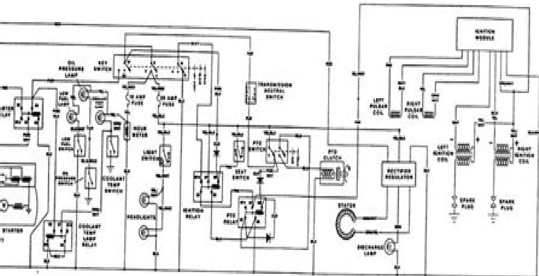
—Wiring diagram for Model 285 with carbureted engine. Refer to Fig. JDS-10 for fuel injection wiring diagram.
