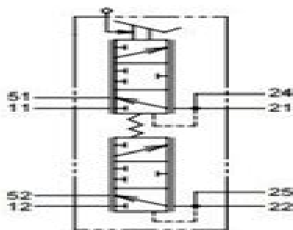
Hydraulic circuit
