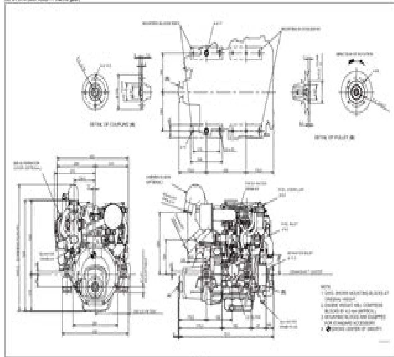
(B) 2Y100 (with H&P-1 marine gear)
