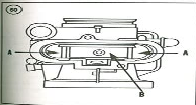
FLOAT LEVEL ADJUSTMENT (1994-1996 MODELS)
