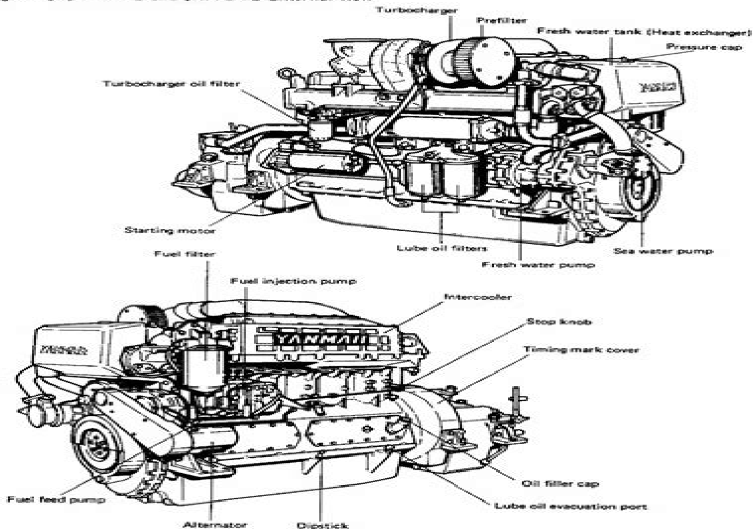
Fig. GI-5. 6HA-HTE and 6HA-DTE External view
