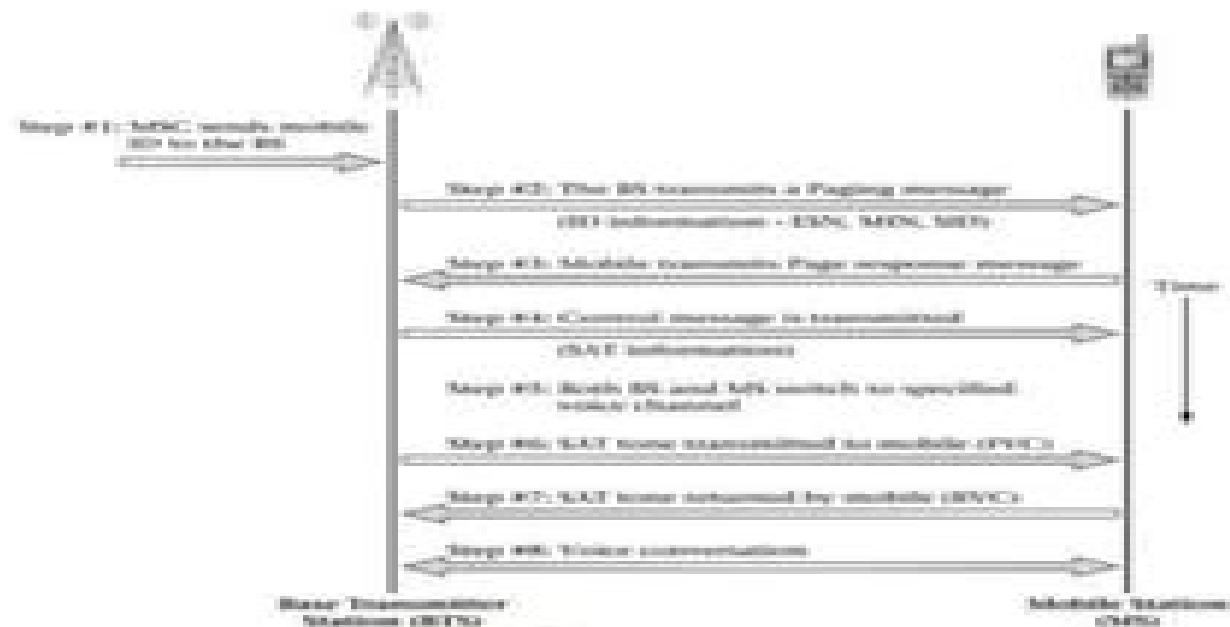
Figure 2.13: AMPS Mobile Terminated call
