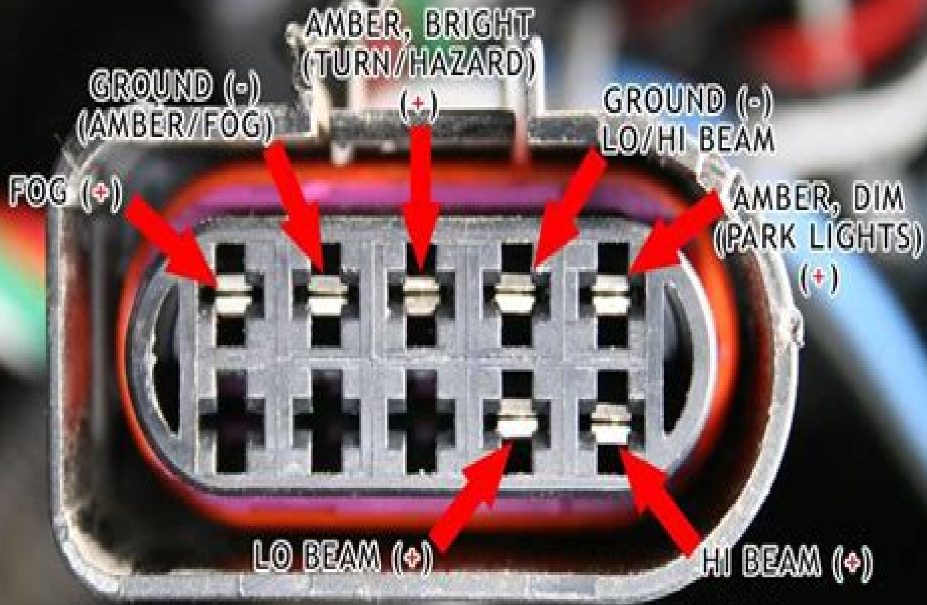
U.S. / NORTH AMERICAN SPEC VOLKSWAGEN MKIV GOLF/JETTA HEADLIGHT HARNESS (CAR SIDE)
