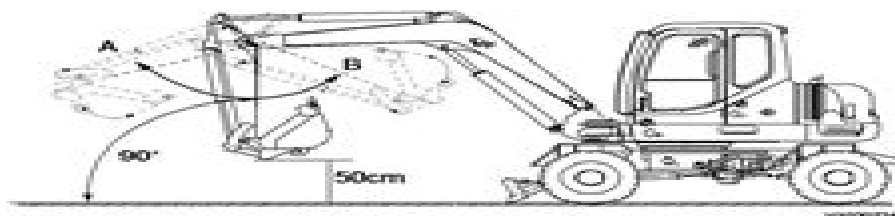
Figure 2 Measuring condition, arm cylinder
