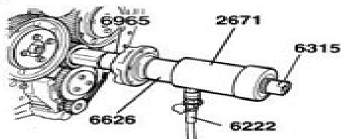
Fig. 14: Installing polygon hub
