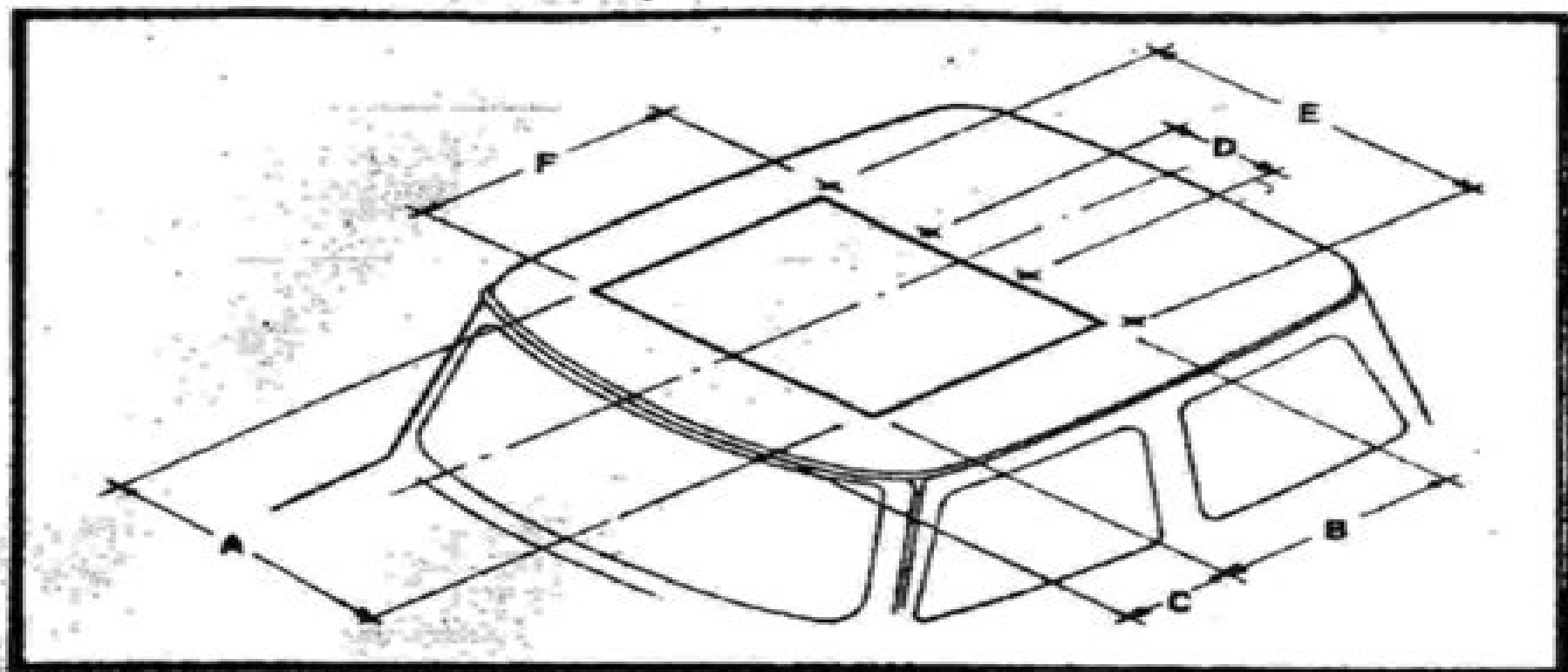
Fig. 1. Dimensions for Templates
