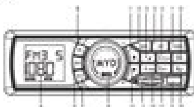
Figure 66-3 Media Player
