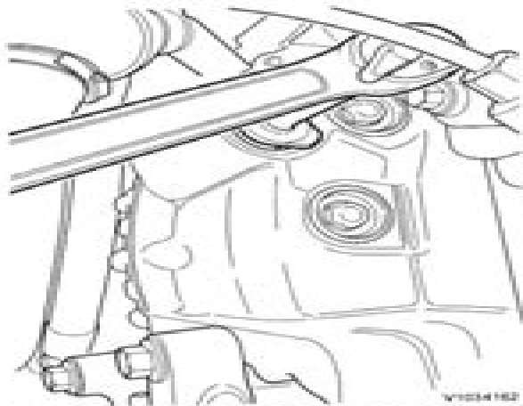
Fig. 151 9993590, extension and ratchet handle
