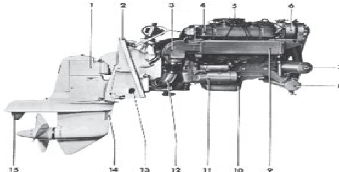
Fig. 1 AQ150/200, viewed from the starboard side
