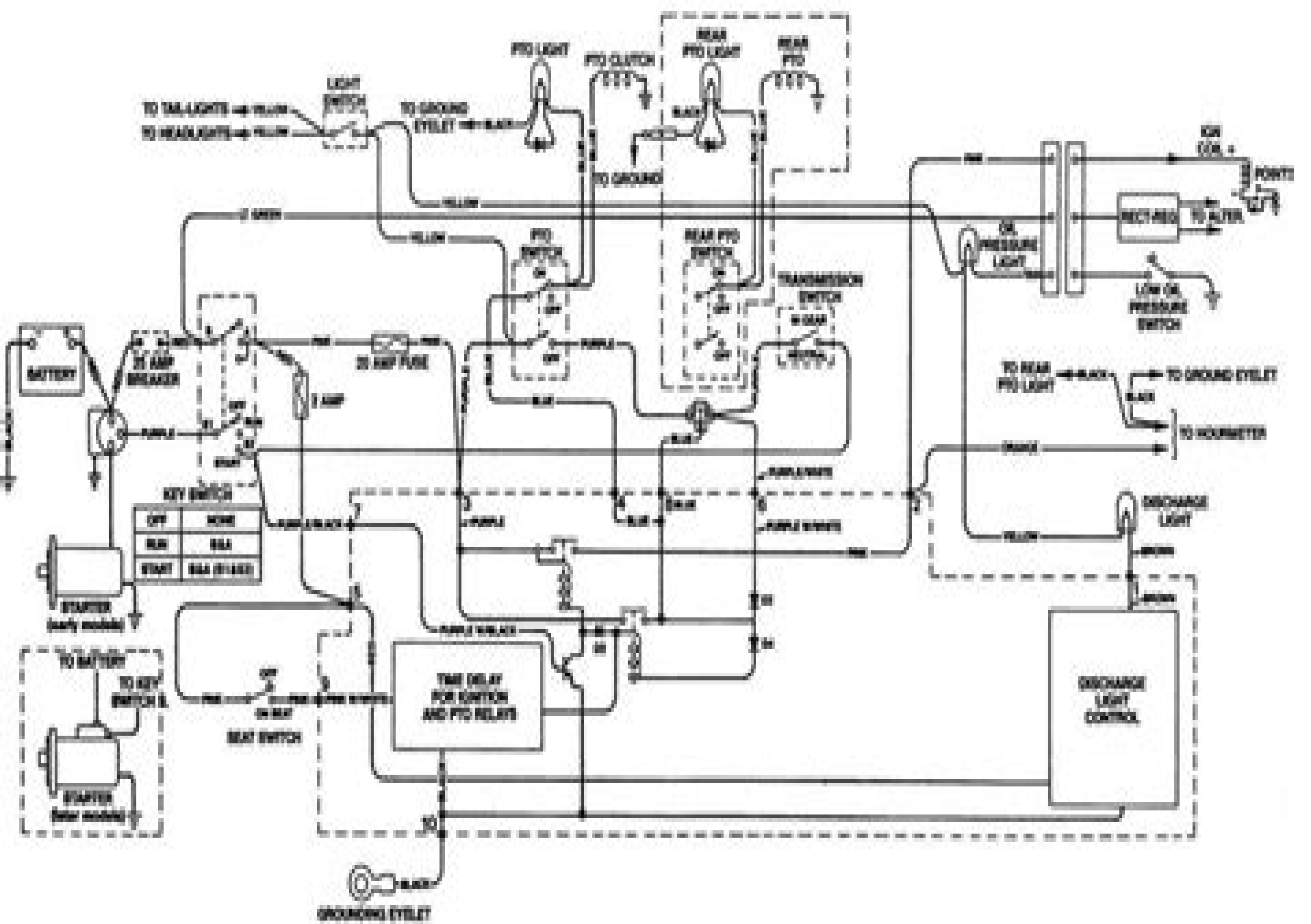
46-22-Wiring diagram for Model 316.
