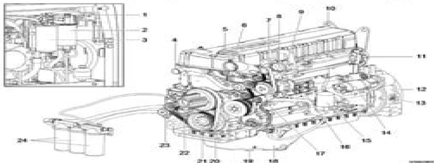
Figure 2 Engine, structure
