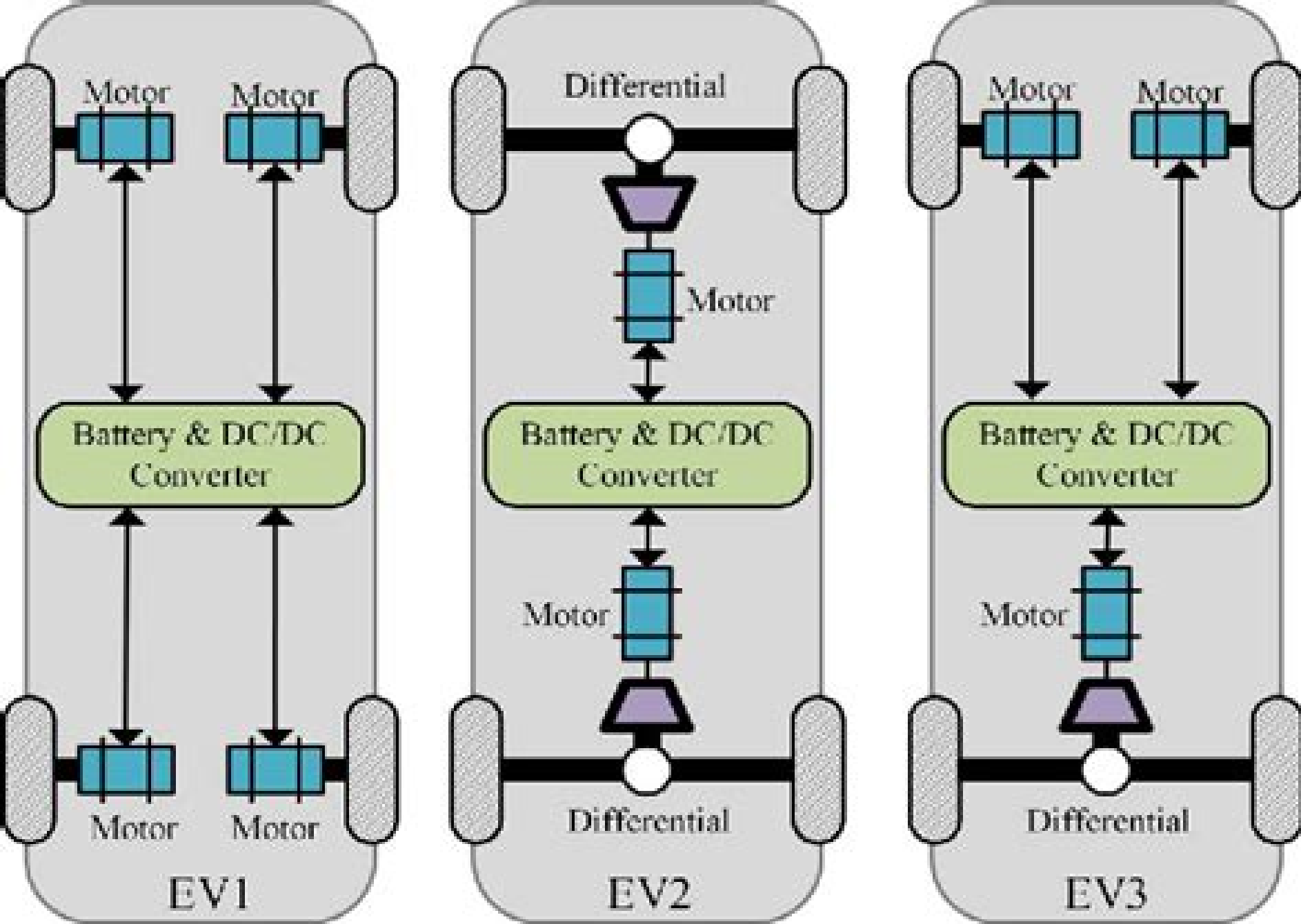
Fig. 1. Different EV propulsion system configurations
