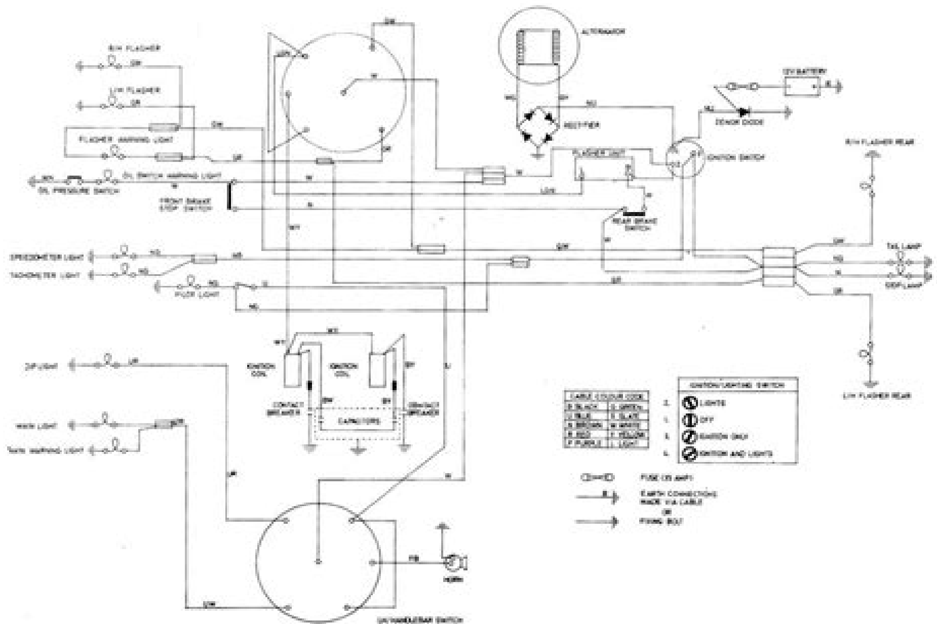
Schematic wiring diagram of a 650cc Triumph 1971 model, up to Engine No. HG36870.
