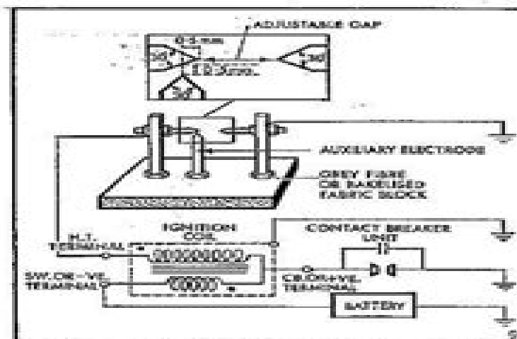
Fig. H3. Ignition coil test rig
