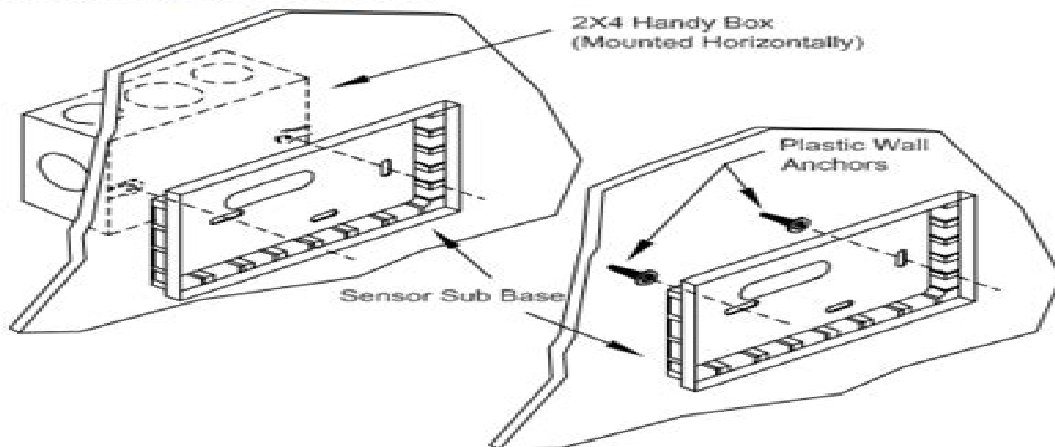
Figure 2 Mounting the Sub Base
