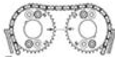
Camshaft to Cylinder Head Alignment Marks
