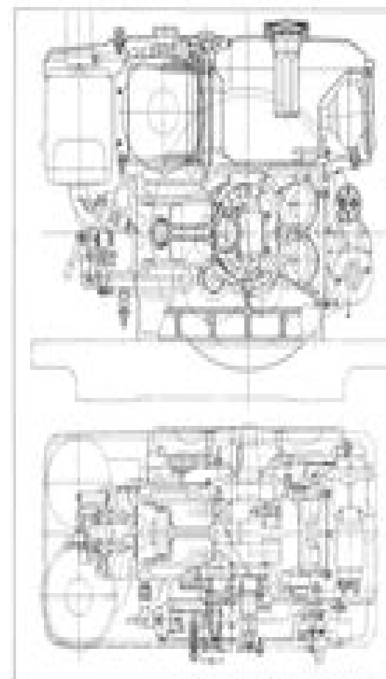
Figure 2-1 Sectional Views
