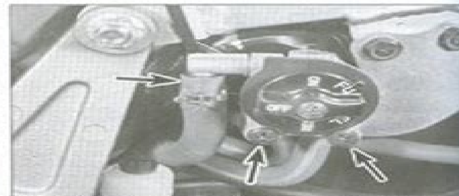
2.11a. Remove the hose and the mounting screws (arrows) ...
