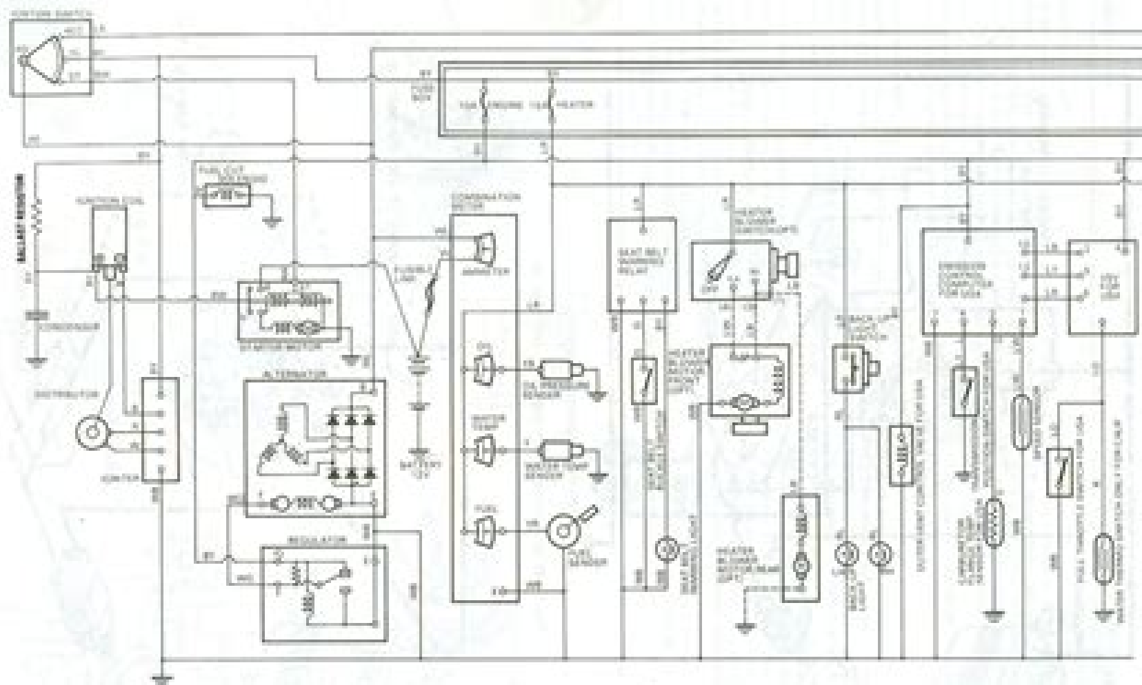
Fig. 13.47 Wiring diagram — FJ 40 series (USA and Canada) 1978
