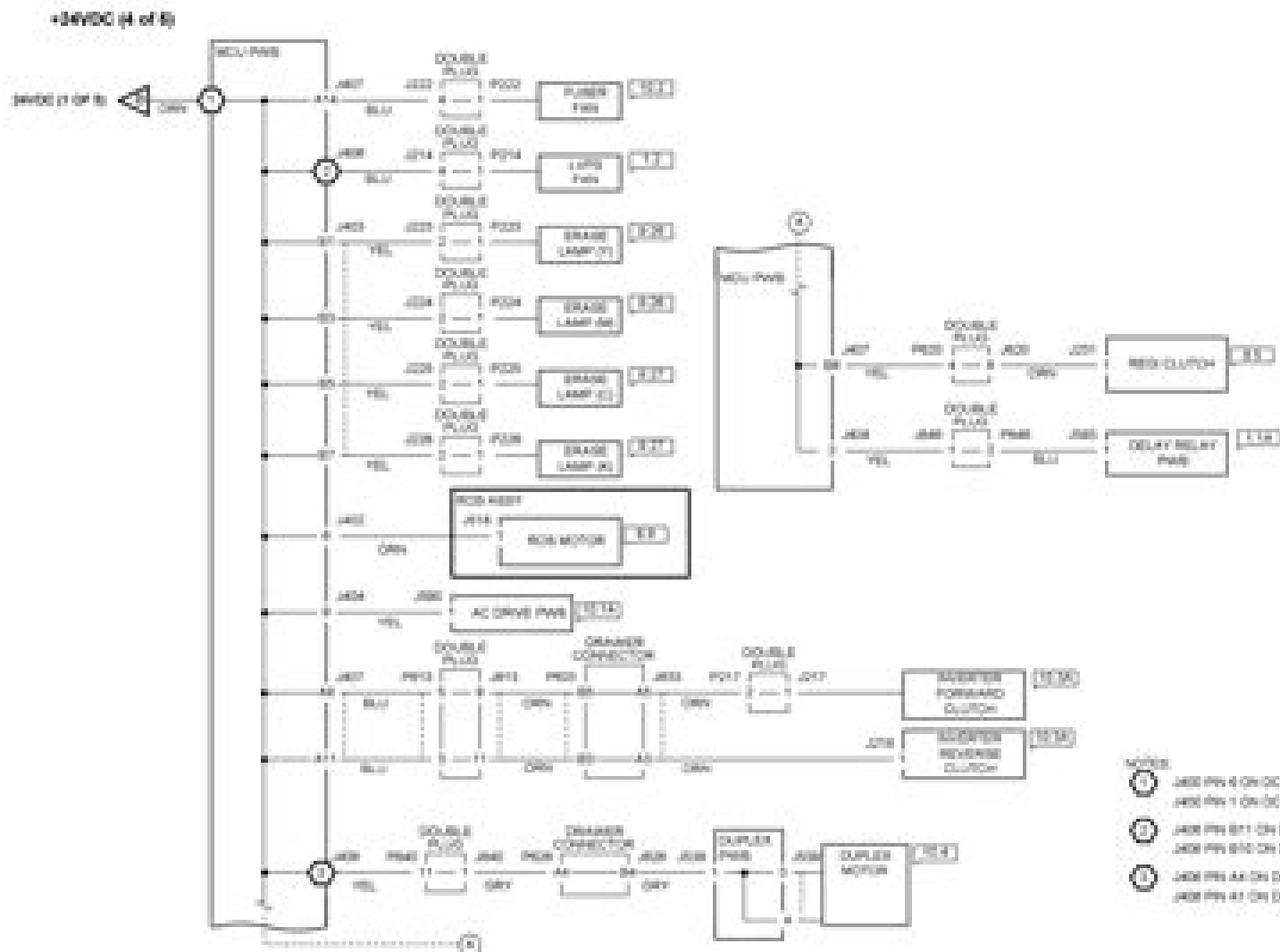
Figure 4 +24VDC (4 of 5) Wirenet
