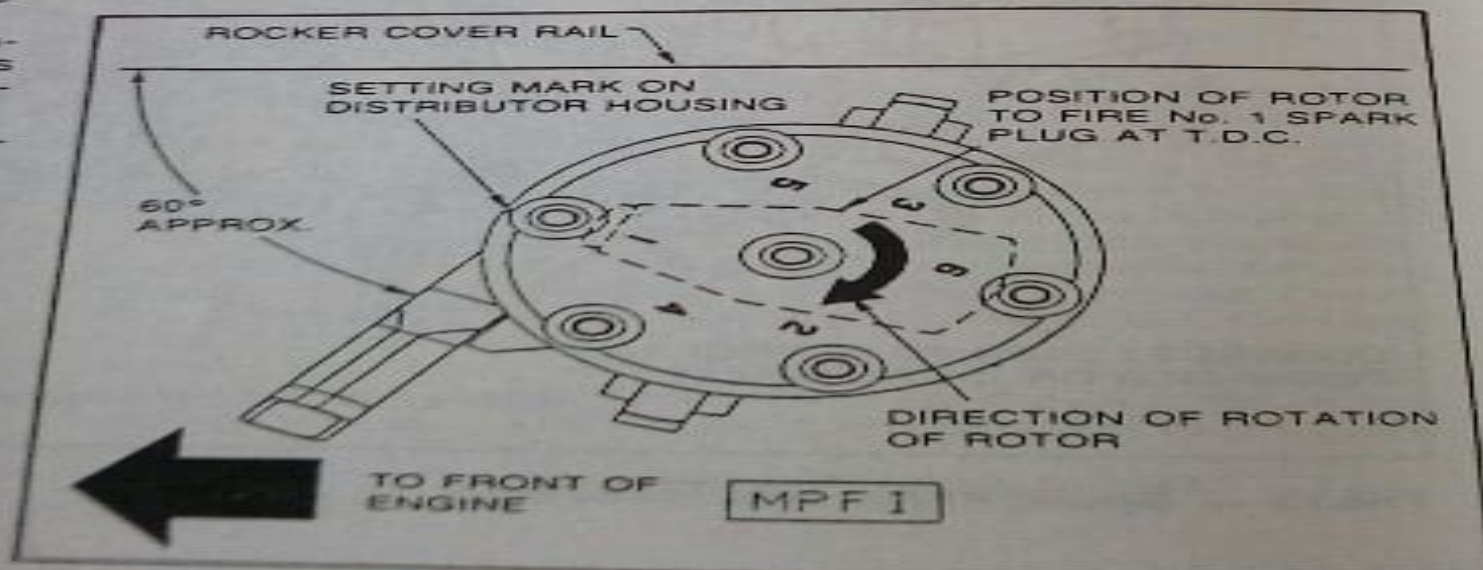
FIG.15 — Distributor Installation — M.P.E.F.I.
