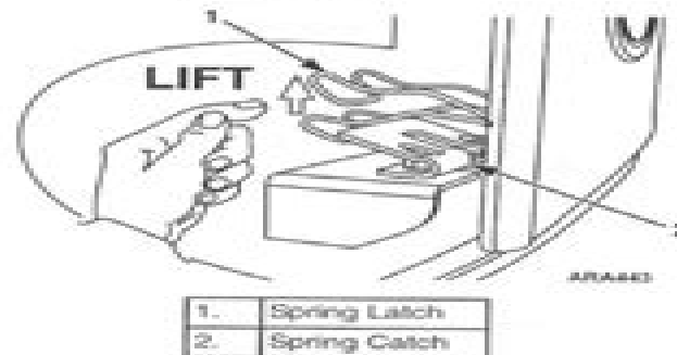
Figure 7: Opening Secondary Door Latch
