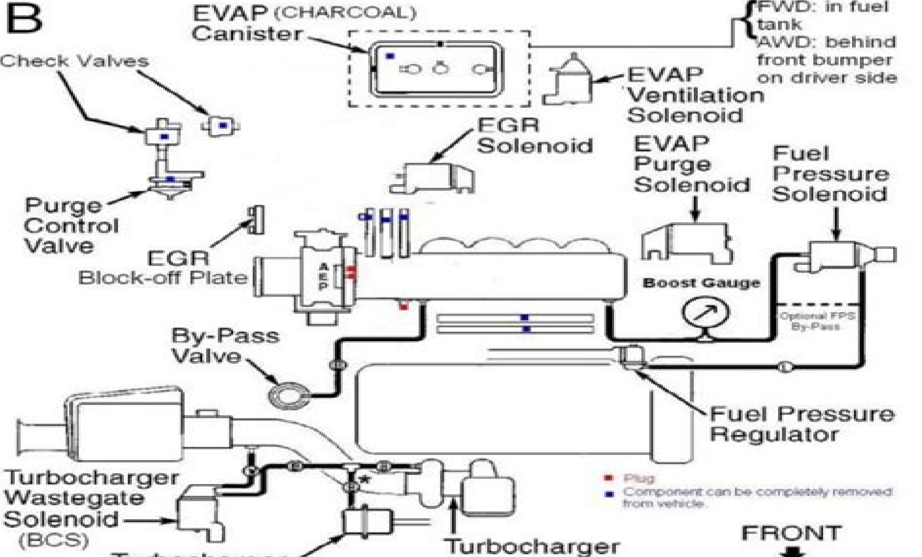
1998-1999 4G63 Vacuum Diagram (with main vacuum reduction)
