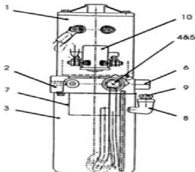
Figure 41 Hydraulic Motor, Pump, and Reservoir
