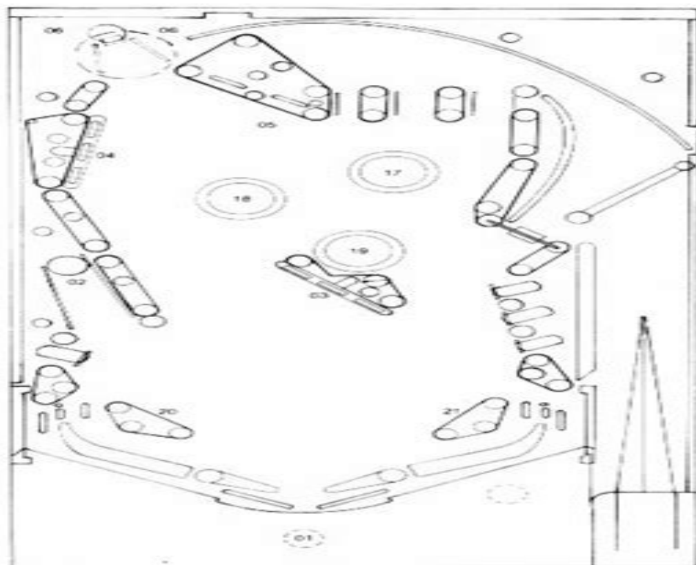
Figure 3. Playfield Solenoid Locations and Solenoid Chart
