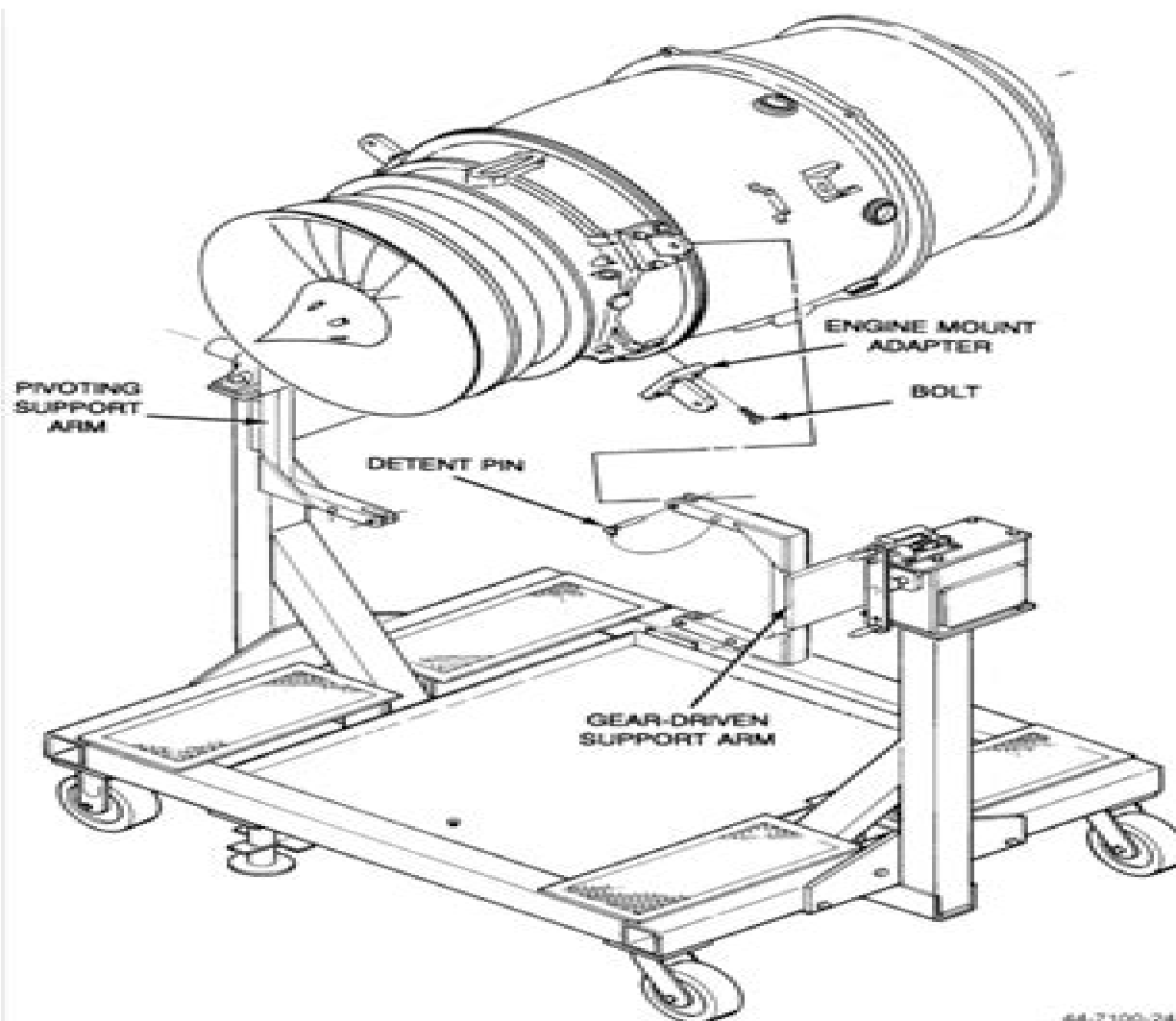
Fig. 401 Engine in Build Stand - Removal/Installation
