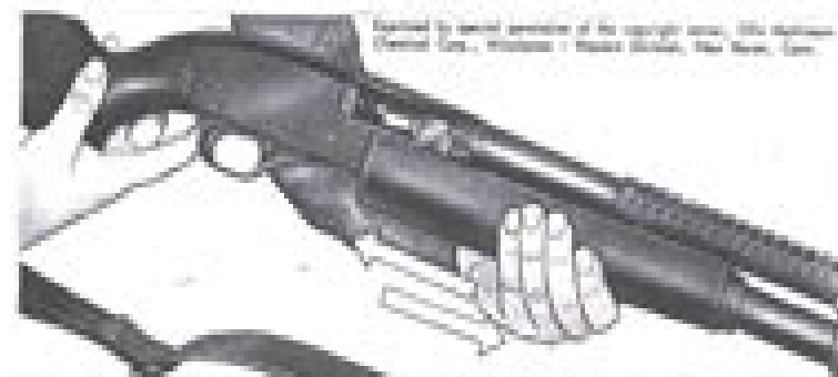
FIG. 4. DEPRESS INTERCONNECT ASSEMBLY AND PRESS FIRE BAR TO CHAMBER ONE CARTRIDGE. HOLD FIRE CARTRIDGE IN CHAMBER.
