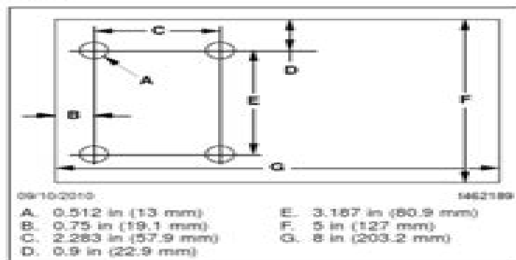
Fig. 1. Holding Fixture Template
