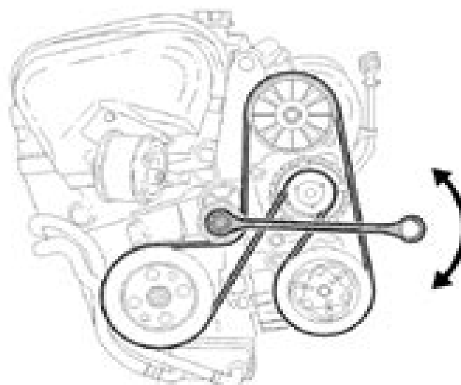
Fig. 16. Removing/Installing Drive Belt
