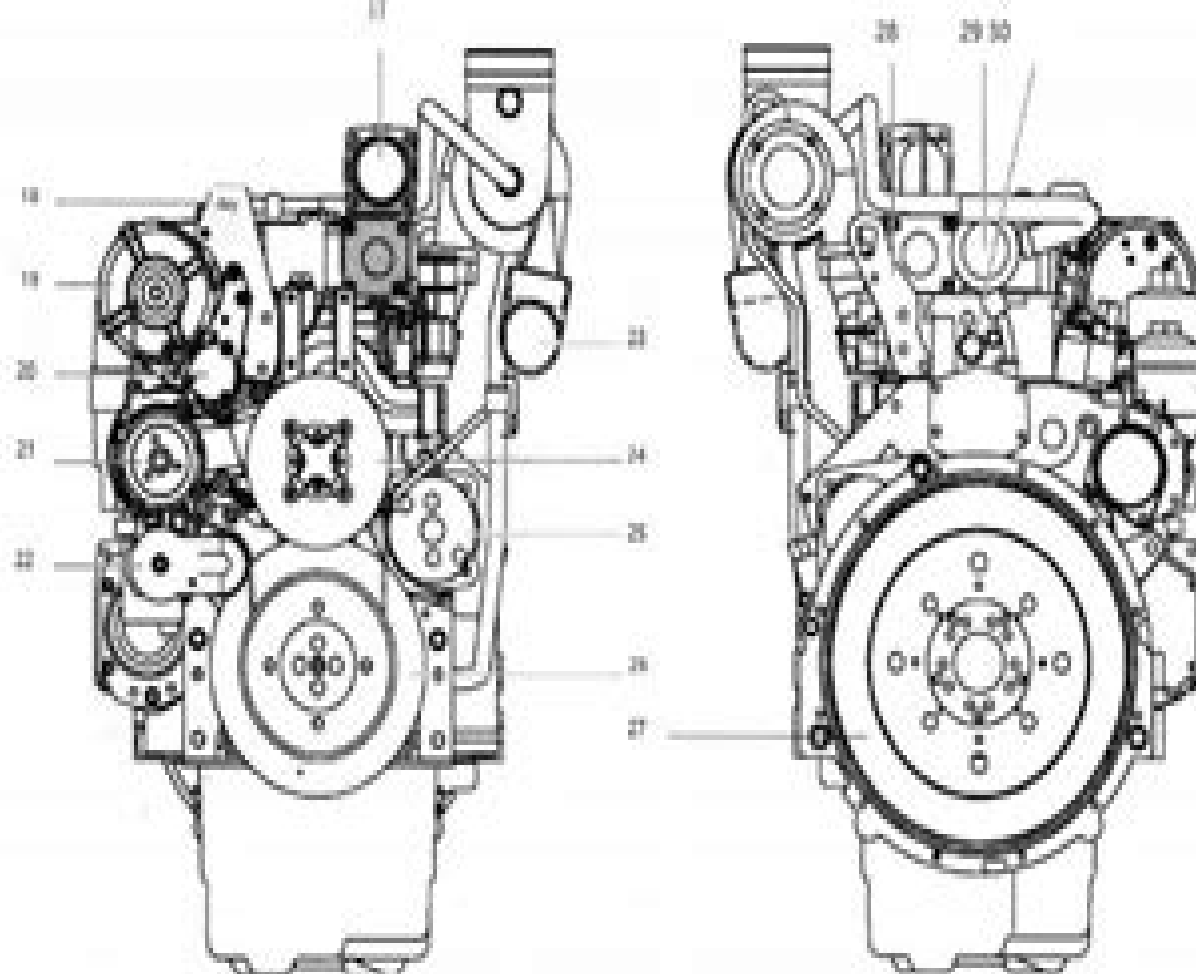
Figure 2-1 Engine, starting motor side view
