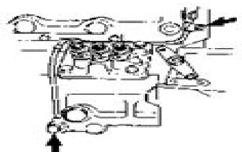
Fig. 12. Dismantling of oil pressure pipe (cylinder block - cylinder head/rocker mechanism)
