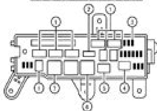
801 ENGINE ROOM RELAY BLOCK NO.1
