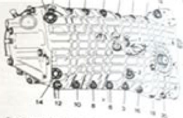
Fig. 6.18 Tighten casing bolts in the sequence shown (Set)
