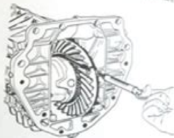
Fig. 6.19 Method of checking bearing preload adjustment (Set)
