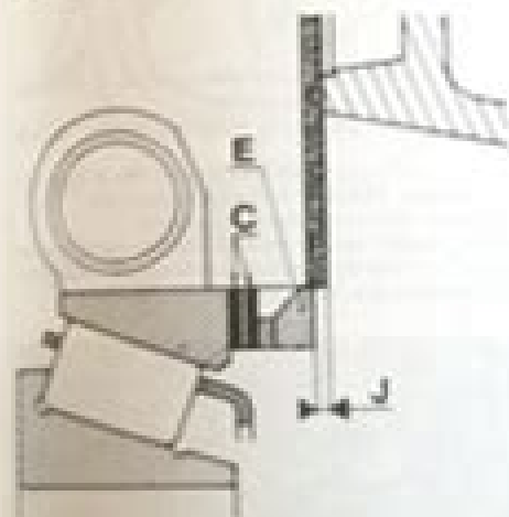
Fig. 6.22 Check the primary shaft endfloat (only 367 model). Clearance at J must be as specified (See 6)
