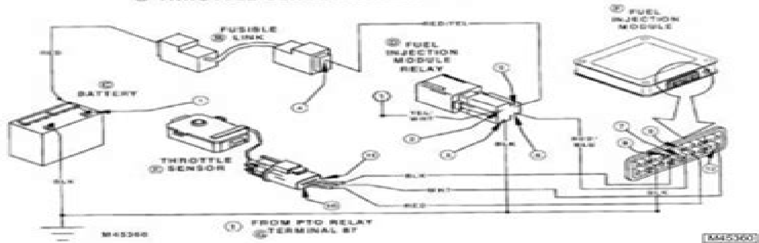
② THROTTLE SENSOR CIRCUIT VOLTAGE TEST
