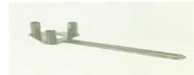
This tool is used to hold the clutch when removing or installing the clutch nut.
